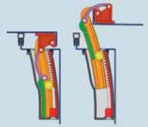
Gear hinge with moving pivot point for high load
